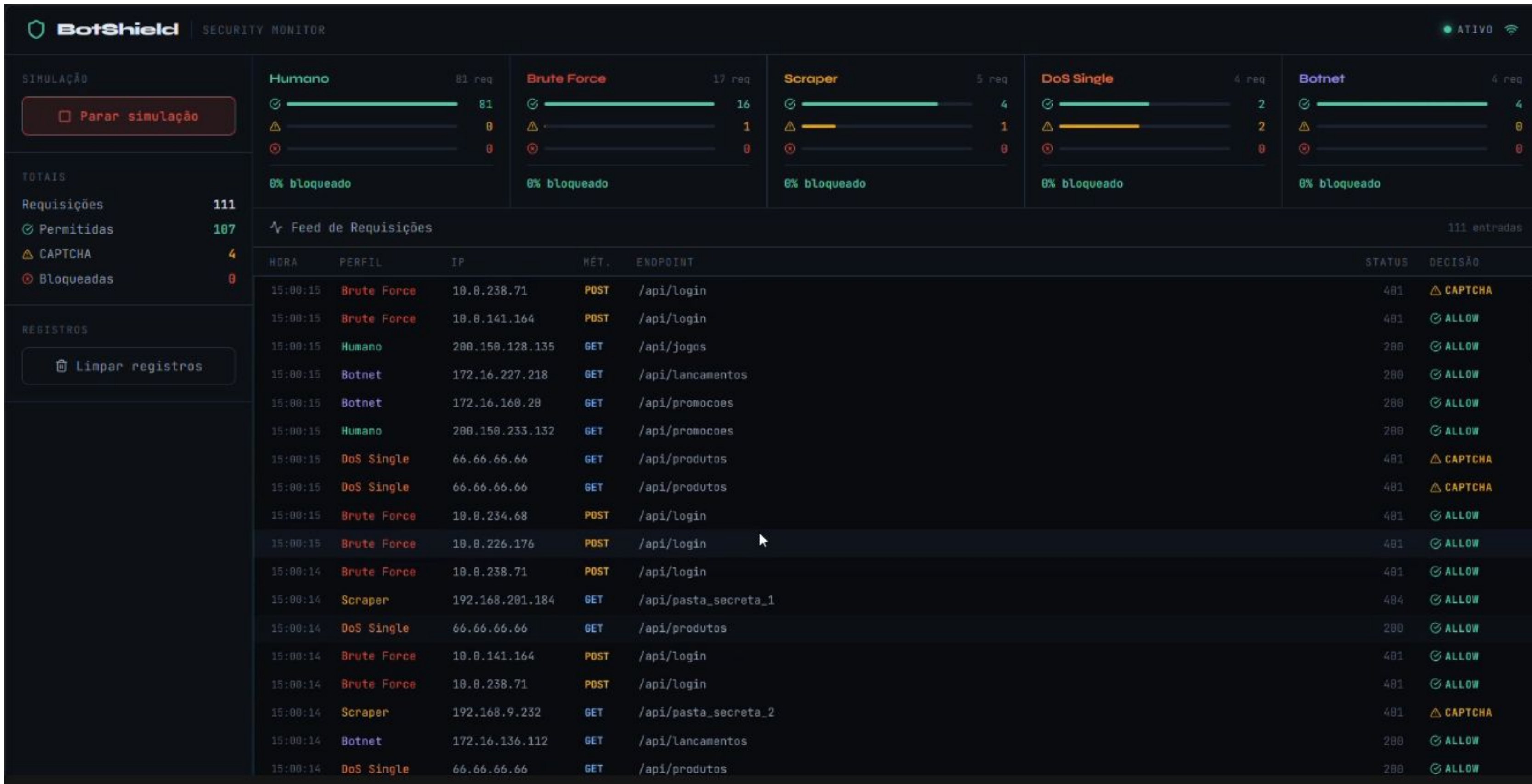
Figura 2 – Features Importantes
